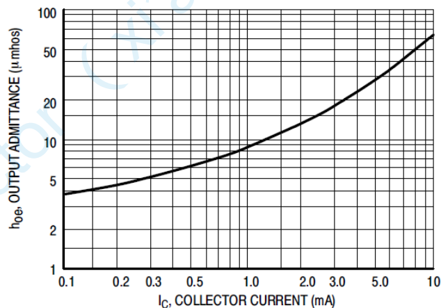
Figure 10. Output Admittance
