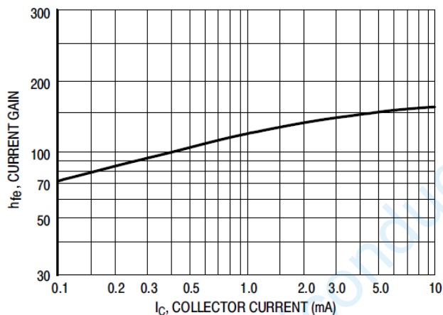
Figure 9. Current Gain
