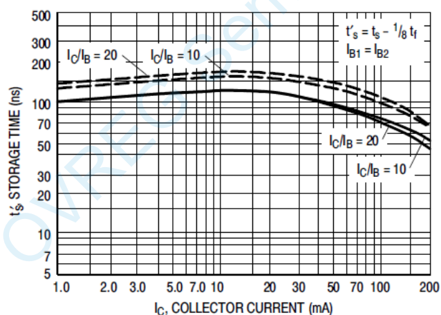
Figure 5. Storage Time
