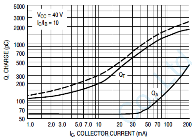
Figure 2. Charge Data
