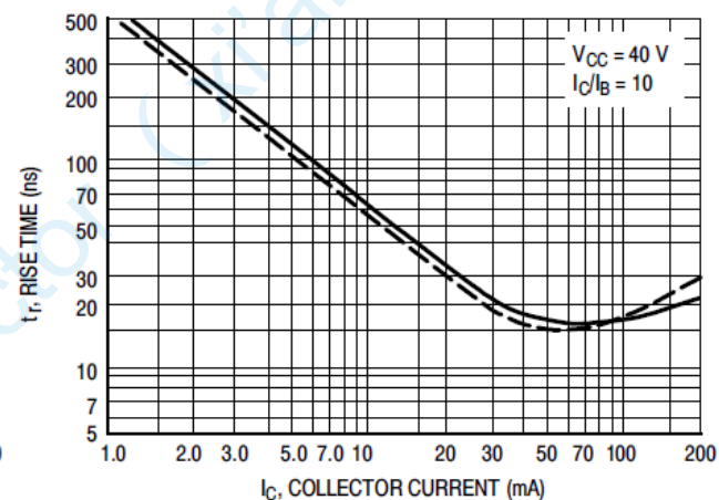
Figure 4. Rise Time
