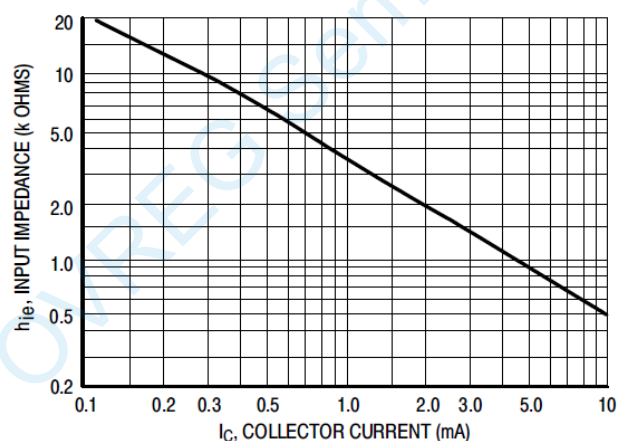
Figure 11. Input Impedance
