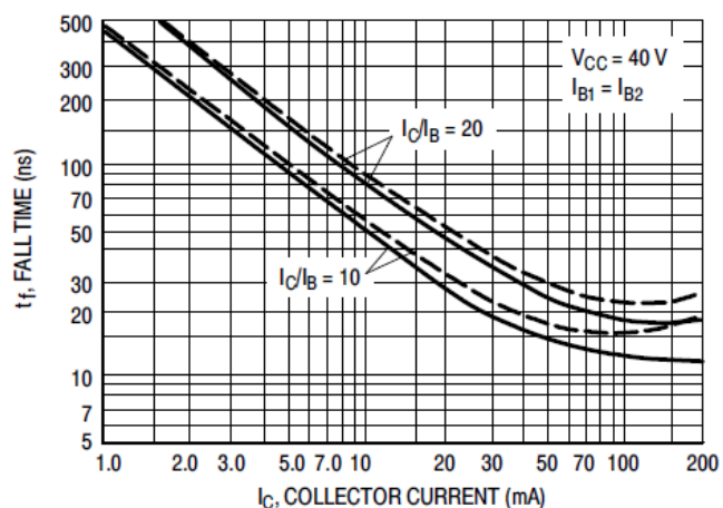
Figure 6. Fall Time
