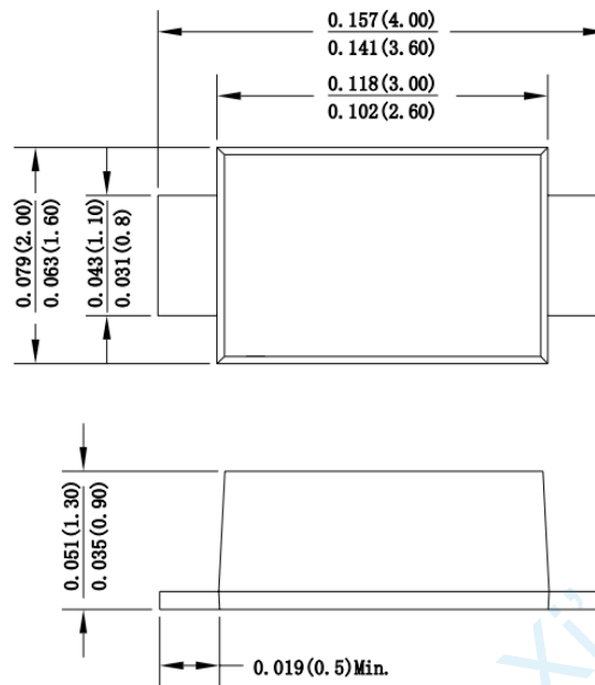
SOD123FL
