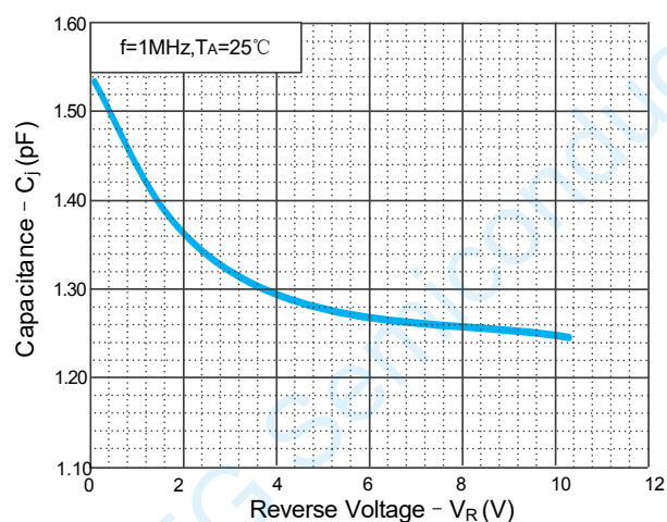
Capacitor Characteristics
