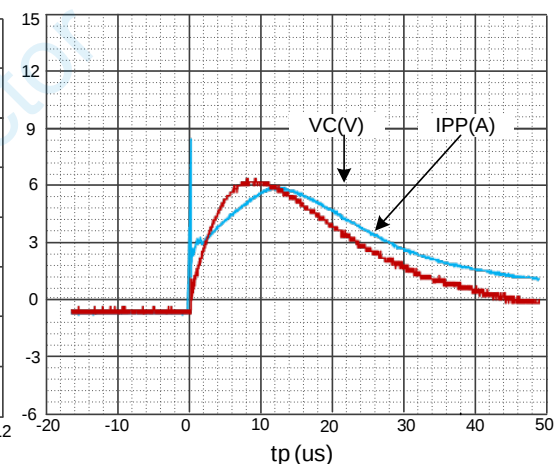
IEC61000-4-5 : 8/20us Waveform
