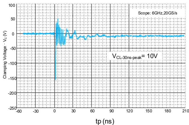
IEC61000-4-2 :15 kV negative pulse from pin 1 to pin 2
