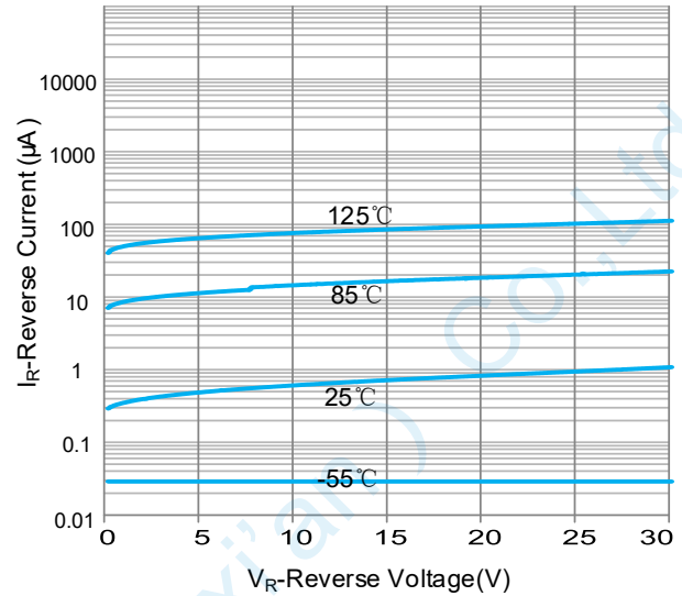
Reverse Characteristic
