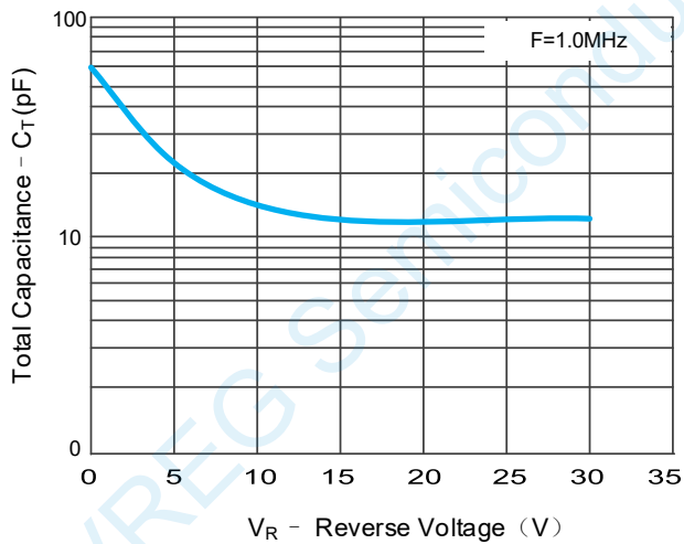
Capacitor Characteristics
