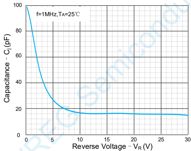
Capacitor Characteristics
