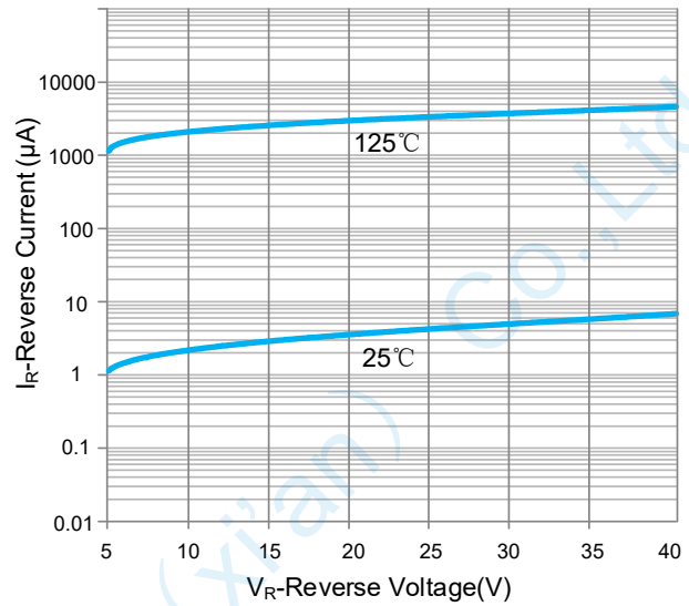
Reverse Characteristic
