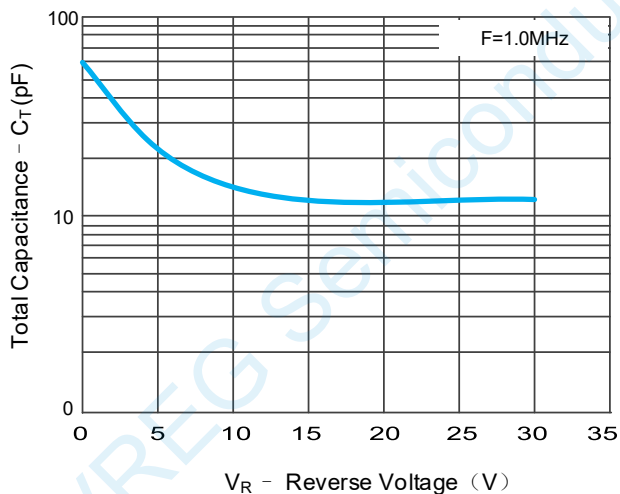
Capacitor Characteristics
