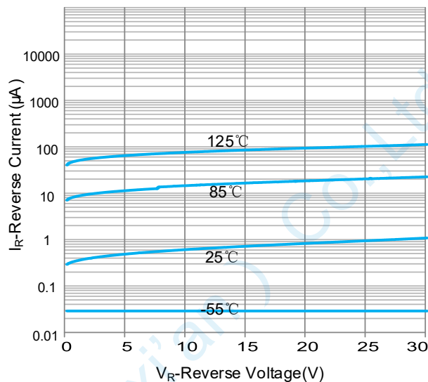
Reverse Characteristic
