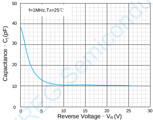
Capacitor Characteristics
