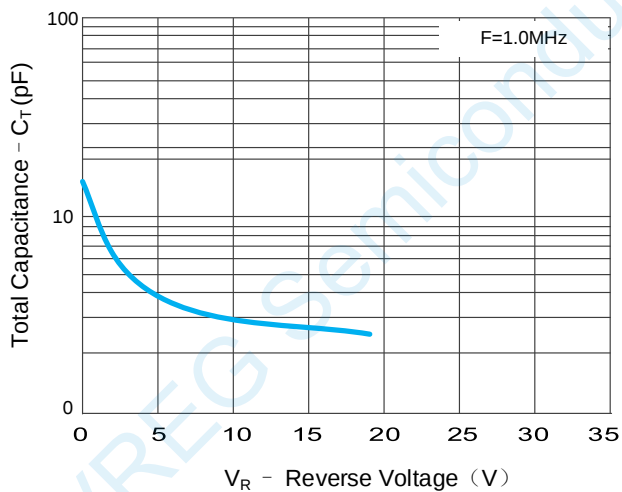
Capacitor Characteristics
