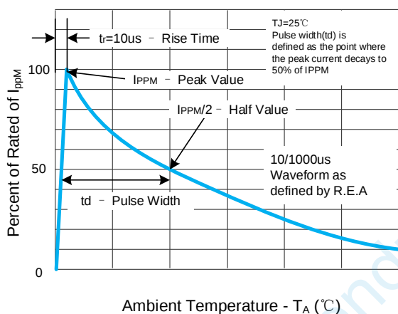
Pulse Waveform
