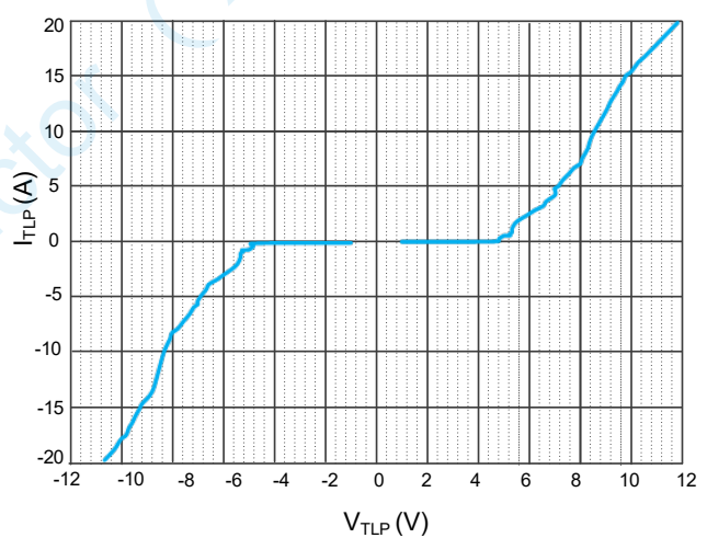
TLP Measurement
